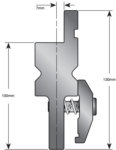
Part No. 43000
