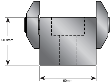
Part No. 43016
