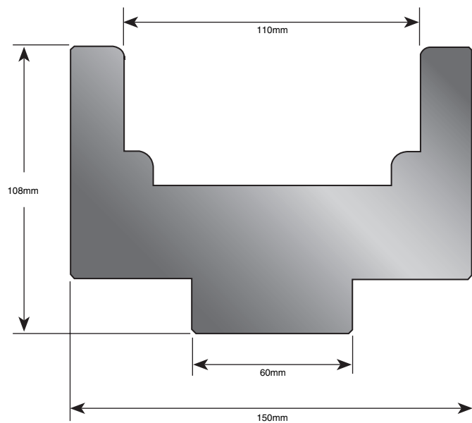
Part No. 42504
