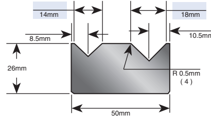
Part No. E42033 90°
