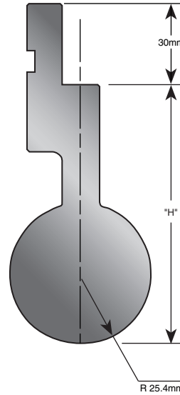
Part No. E41725
