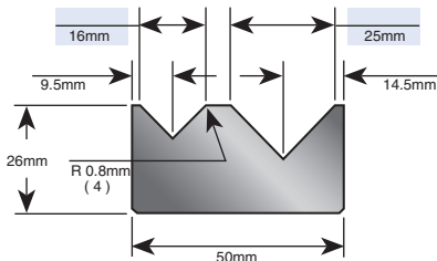
Part No. E42036 88°
