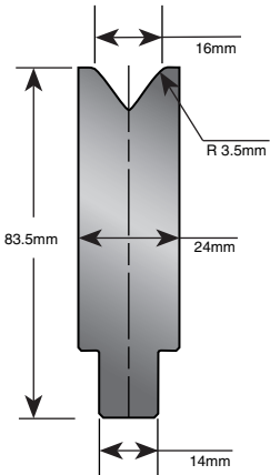
Part No. E44204
