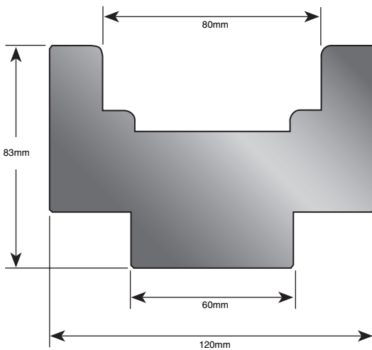
Part No. 42503
