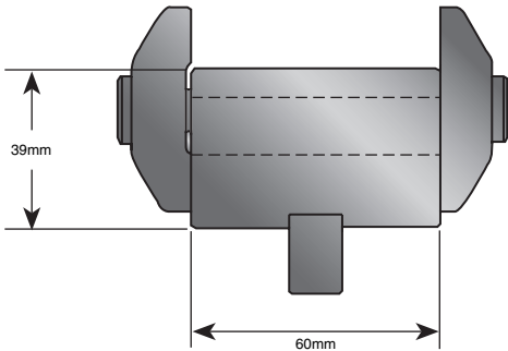
Part No. 43006
