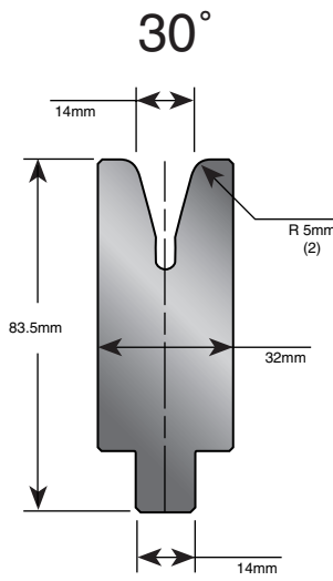
Part No. E42204
