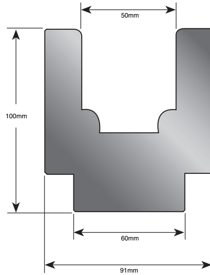
Part No. 42502
