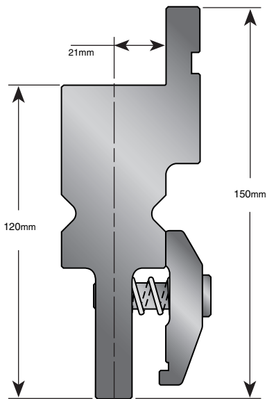
Part No. 43001
