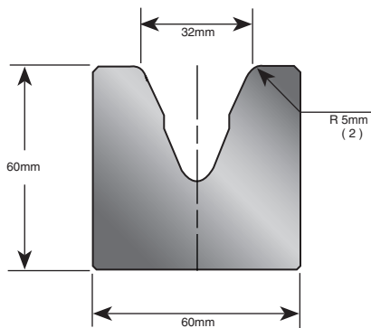
Part No. E42302
