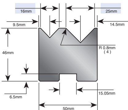
Part No. E42056 88°
