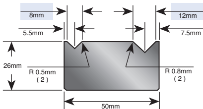
Part No. E42032 90°
