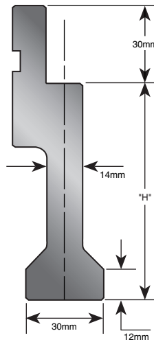
Part No. E41630
