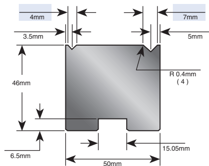
Part No. E42050 90°
