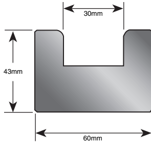
Part No. 42501
